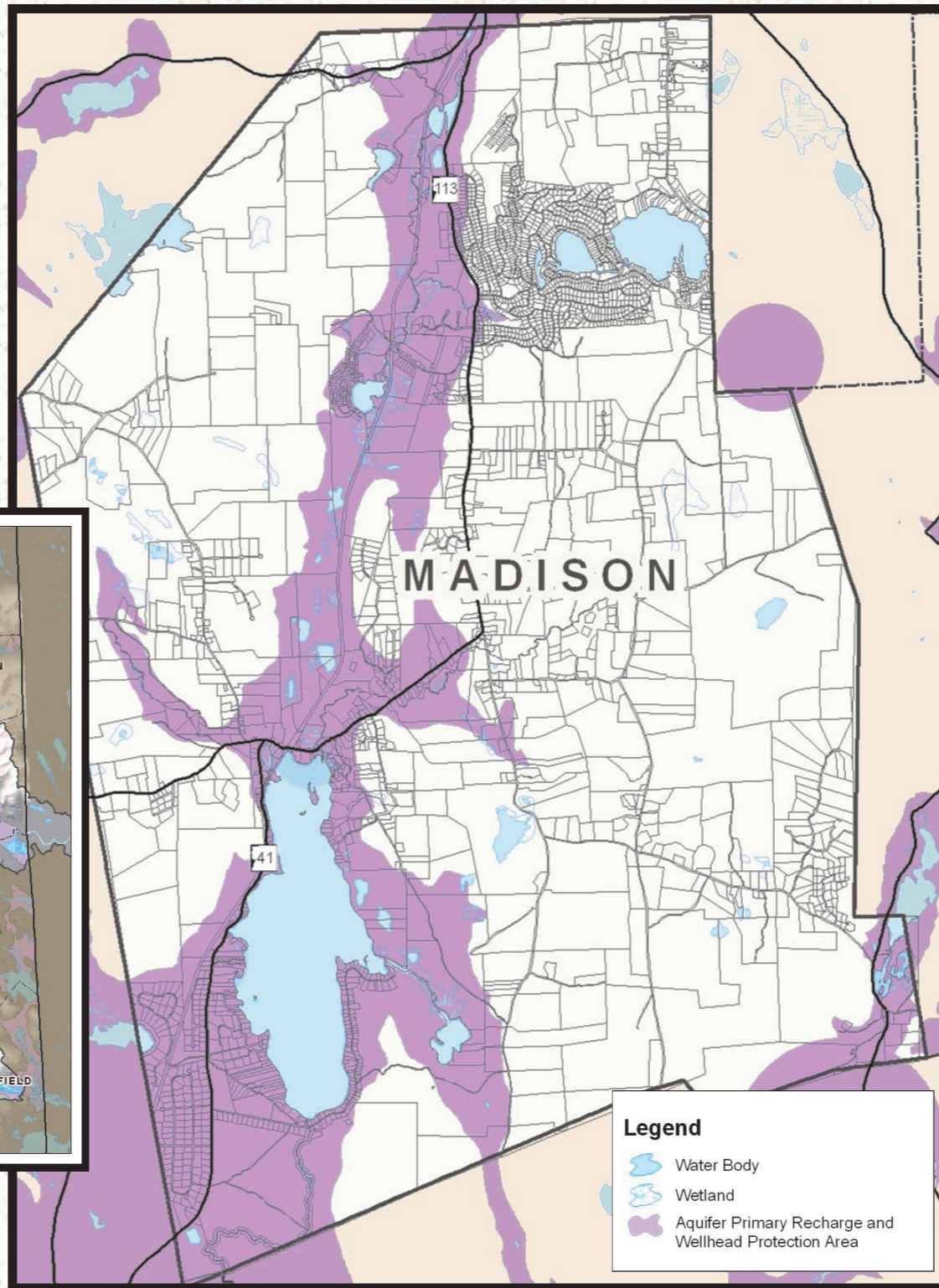
Maps created by Lakes Region Planning Commission of geohydrology and water quality of stratified-drift aquifers in the Saco and Ossipee River basins, East-Central New Hampshire, USGS Water-Resources Investigations Report 94-4182.
