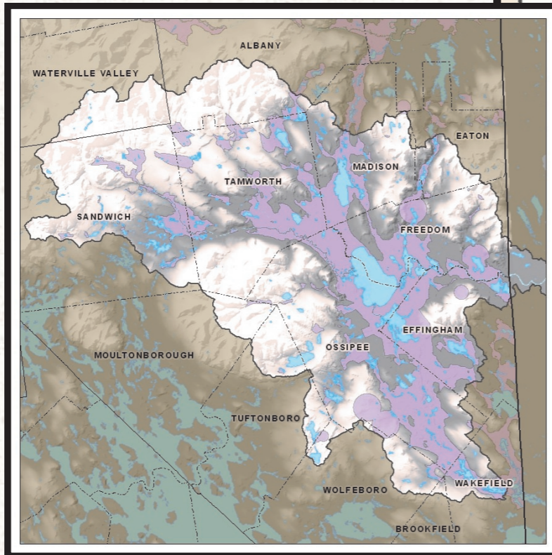
Maps created by Lakes Region Planning Commission of geohydrology and water quality of stratified-drift aquifers in the Saco and Ossipee River basins, East-Central New Hampshire, USGS Water-Resources Investigations Report 94-4182.
