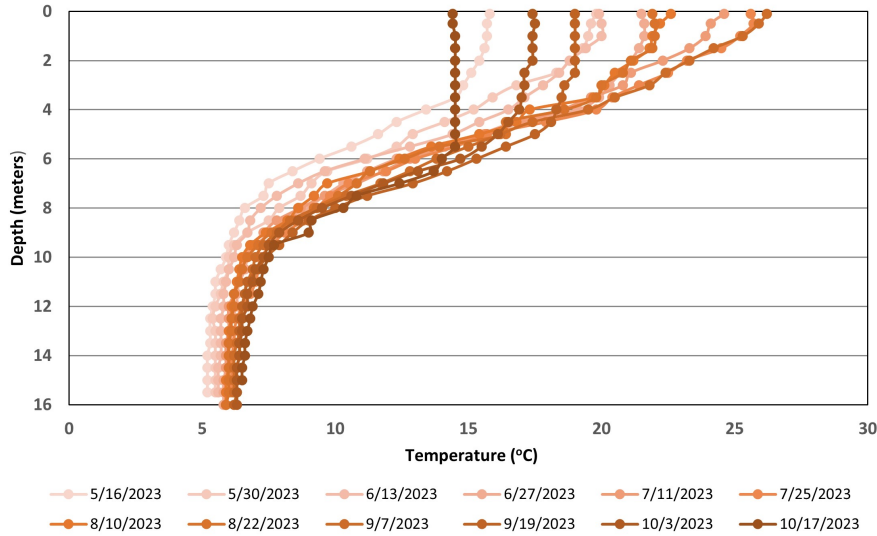
Figure 6. Loon Lake - Site Deep Temperature Profiles (May 16 through October 17, 2023)
