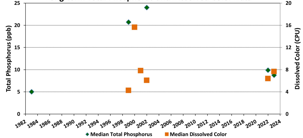
Figure 5. White Pond - Deep Site (1983-2023) Long-term Total Phosphorus and Dissolved Color Data
