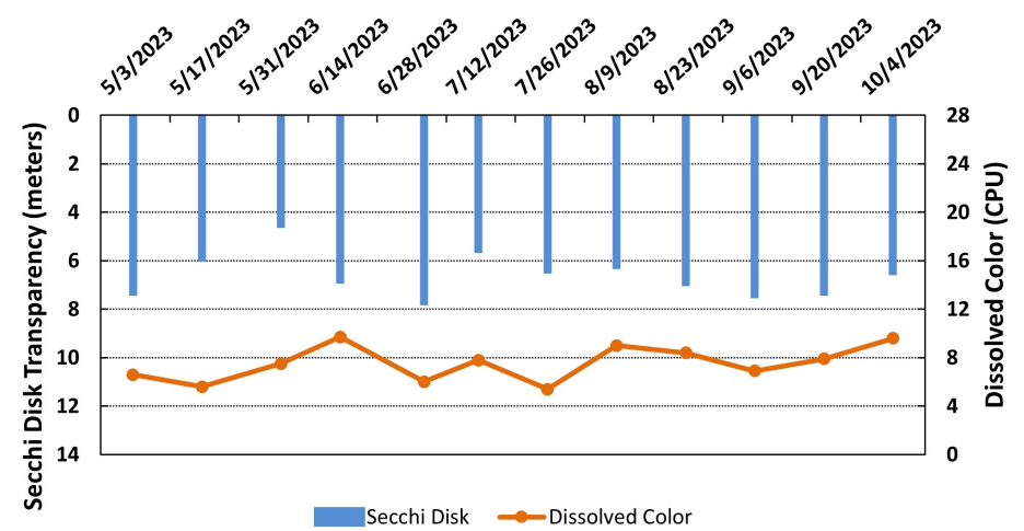
Figure 3. White Pond (2023 Seasonal Data) Secchi Disk Transparency and Dissolved Color Data
