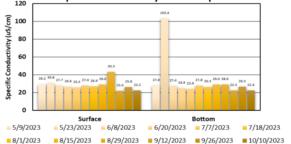
Figure 9. White Pond - Site Deep Specific Conductivity inter-comparison
