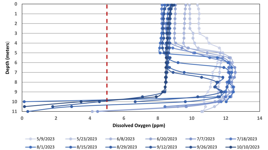
Figure 7. White Pond - Site Deep Dissolved Oxygen Profiles (May 9 through October 10, 2023)
