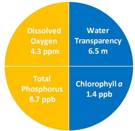
Figure 1. White Pond Water Quality (2023)
