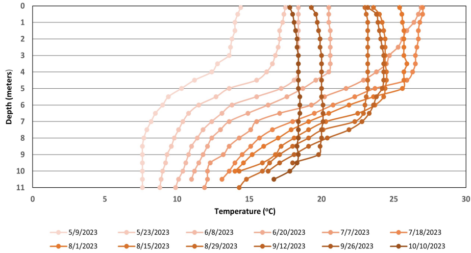
Figure 6. White Pond - Site Deep Temperature Profiles (May 9 through October 10, 2023)
