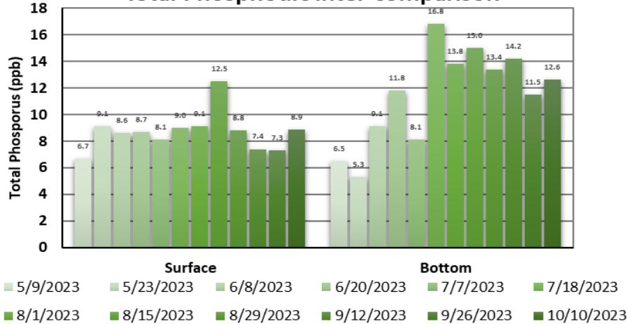
Figure 8. White Pond - Site Deep Total Phosphorus inter-comparison
